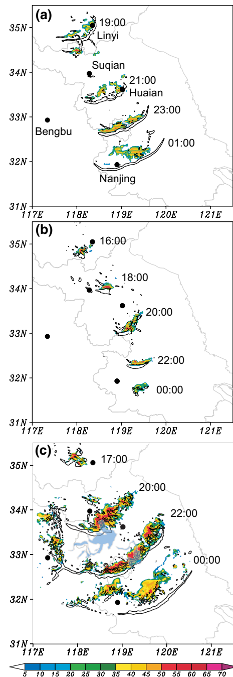
Fig. 10 a The radar reflectivity (shading, dBZ) simulated in EXP-M at 3 km with the updraft of 1 \text{ m s}^{-1} (contours) at 1 km AGL. b and c are the same as a , but for the EXP-L1 and EXP-L2, respectively
