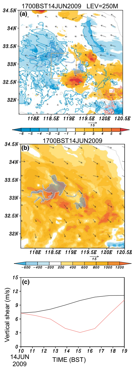
Fig. 12 a The difference of 250-m temperature (shading, K) and water vapor mixing ratio (contours, \text{g kg}^{-1} ) between EXP-C and EXP-L1, and 250-m winds (vectors, \text{m s}^{-1} ) in EXP-C at 1700 BST. b The difference of CAPE (contours, \text{J kg}^{-1} ) between EXP-C and EXP-L1 and winds (vectors, \text{m s}^{-1} ) at 3 km in EXP-C at 1700 BST. Blue shading highlights Hongze Lake and Gaoyou Lake. c The time series of vertical wind shear between 0.25 km and 3 km in EXP-C (black line, \text{m s}^{-1} ) and EXP-L1 (red line, \text{m s}^{-1} ), respectively. The vertical wind shear is averaged over the orange box in a
