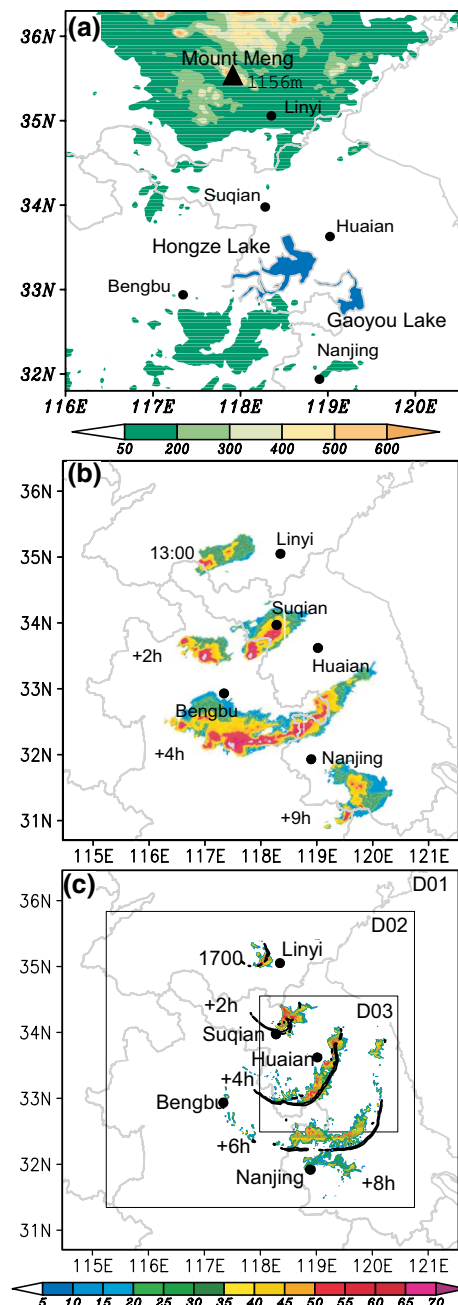
Fig. 1 a Terrain altitude (shading, m) in the region of the squall line activity with the blue shading indicating the lakes. b Observed radar reflectivity (shading, dBZ) at 1300, 1500, 1700, 2200 BST 14 June 2009. c Horizontal grids used for numerical simulations of quasi-linear convective systems on 14 June 2009. In each case, d01, d02, and d03 utilize 3-, 1-, and 0.333-km horizontal grid spacings, respectively. 3-km radar reflectivity simulated in the control experiment. The contours of the updraft of 1 m s -1 at 1 km AGL indicate the approximate location of the gust front. The hours labeled with the system are relative to 1300 BST and 1700 BST 14 June 2009 in b and c , respectively. The black dots are the locations of related cities
