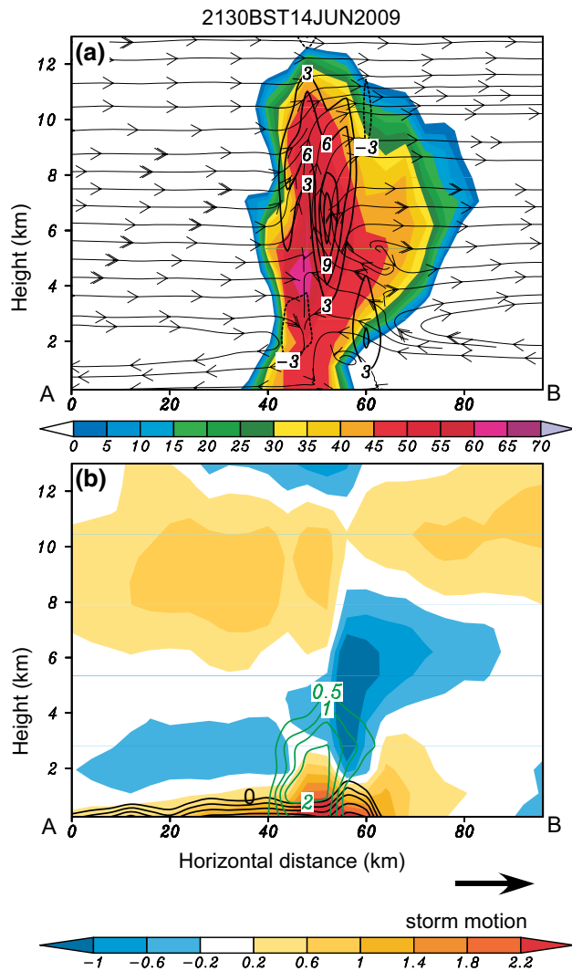
Fig. 5 a Vertical cross-section of radar reflectivity (shading, dBZ), storm-relative flow (streamlines) and vertical motion (contours, \text{m s}^{-1} ) with solid and dash contours indicating upward and downward vertical motion, respectively; b vertical cross-section of the simulated pressure perturbation (shading, hPa) and rain mixing ratio (green contours, 0.5 \text{ g kg}^{-1} ). The cold pool potential temperature perturbation below 0 K is plotted at 1 K intervals (thick black contours). The cross-section is plotted along the line in Fig. 4
