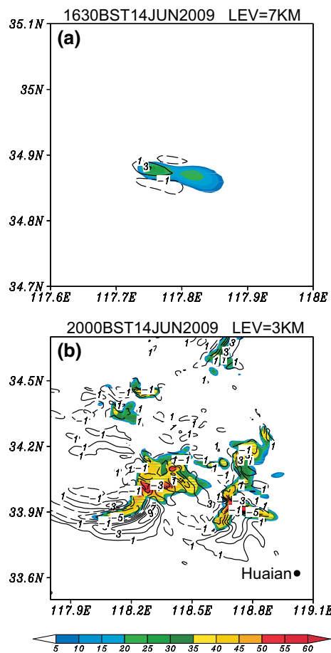
Fig. 11 a The simulated radar reflectivity (shading, dBZ) and vertical motion (contours) at 7 km with solid and dash contours indicating upward and downward vertical motion ( \text{m s}^{-1} ) at 1630 BST 14 Jun 2009 in EXP-M, respectively. b The same as a , but for 2000 BST 14 Jun 2009 at 3 km
