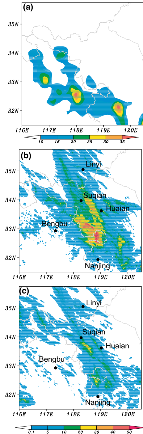
Fig. 6 The accumulate precipitation (shading, mm) from 1700 BST 14 June to 0200 BST 15 June in a observation, b EXP-C and c EXP-M, respectively. The black dots are the locations of related cities
