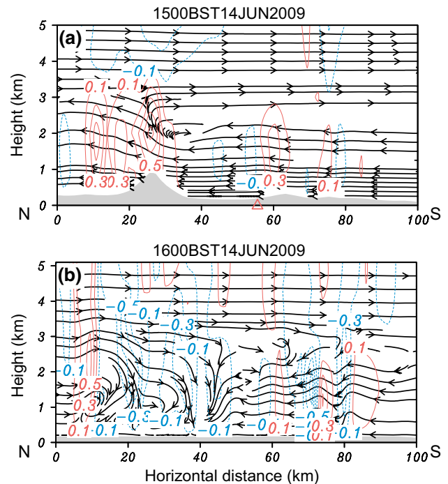
Fig. 8 a The vertical cross-section of the terrain height (shading, m), water vapor mixing ratio (green contours, g kg -1 ), wind (streamlines), and vertical velocity (contours). The red and blue contours indicate the upward and downward vertical motion (m s -1 ) at 1500 BST in EXP-C, respectively. b Same as a , but for 1600 BST in EXP-M. The cross-section is plotted along the line in Fig. 7
