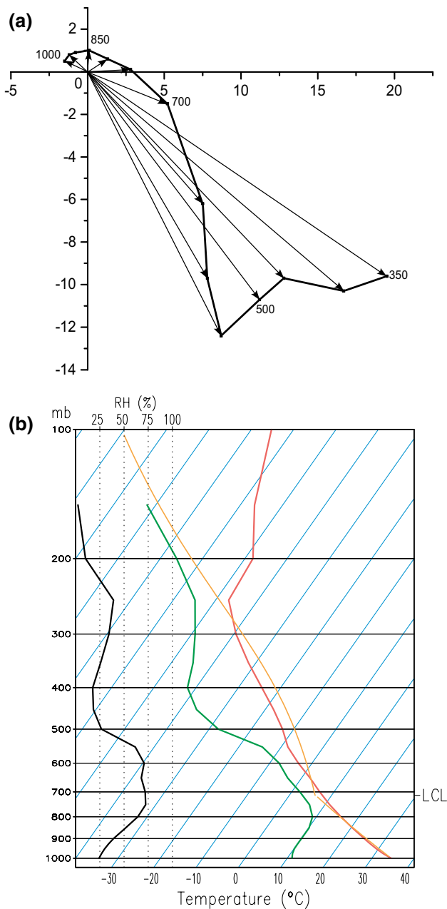
Fig. 3 a The hodograph of average winds (vector, \text{m s}^{-1} ) between 1000 and 350 hPa at 1400 BST 14 June 2009 from the FNL analysis, which are averaged over the orange box in Fig. 2b; b The sounding at 1400 BST 14 June 2009 from the FNL analysis, with the average area being shown in Fig. 2b
