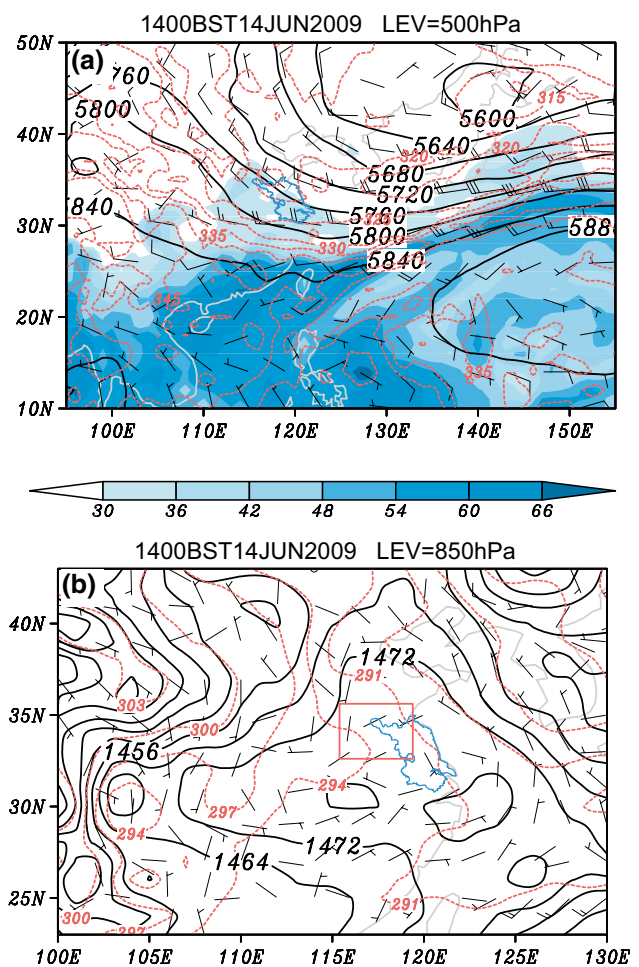
Fig. 2 a The fields of geopotential height (black contours, gpm), potential equivalent temperature (red contours, K), and winds (vectors) at 500 hPa, and column-integrated precipitable water greater than 24 \text{ kg m}^{-2} (shading, \text{kg m}^{-2} ) at 1400 BST 14 June 2009 from the FNL analysis. b The fields of geopotential height (black contours, gpm), equivalent potential temperature (red contours, K), winds (vector) at 850 hPa, and CAPE (shaded, \text{J kg}^{-1} ) from the FNL analysis. The closed blue line outlines the area of Jiangsu Province. The red box indicates the position of the average area in Fig. 3
