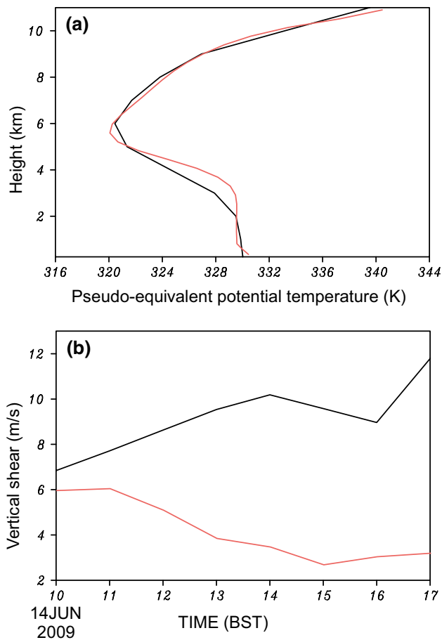
Fig. 9 a The vertical profile of potential pseudo-equivalent temperature in EXP-C at 1500 BST (black) and EXP-M at 1600 BST (red), respectively. b Time-dependent vertical wind shear between 0.25 km and 3 km in EXP-C (black) and EXP-M (red), respectively. The average area for the potential pseudo-equivalent temperature and vertical wind shear is shown in Fig. 7
