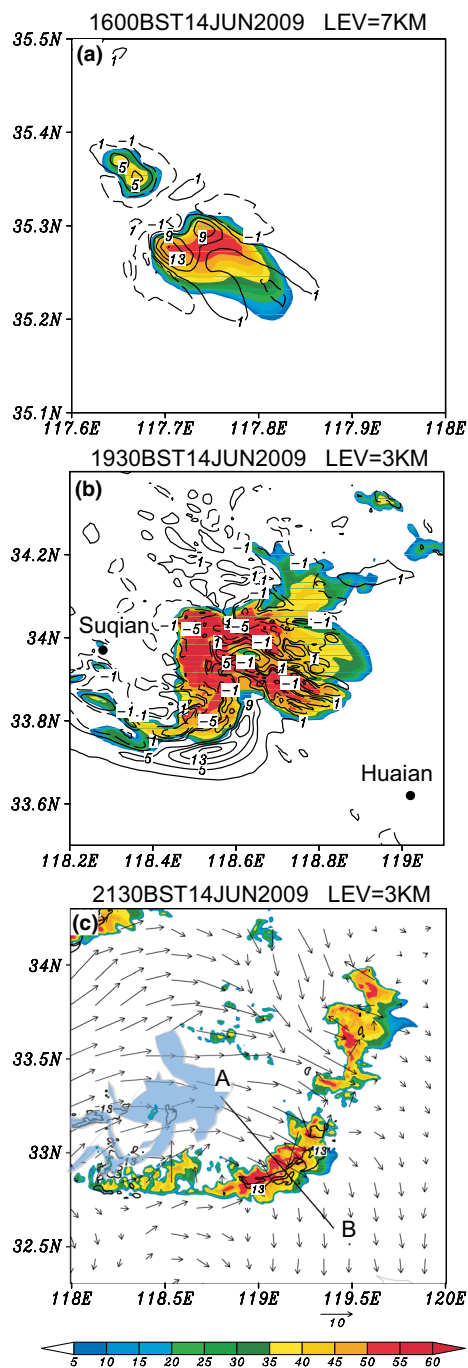
Fig. 4 a The 7-km simulated radar reflectivity (shading, dBZ) and vertical velocity (contours \text{m s}^{-1} ) with solid and dash contours indicating upward and downward vertical motion at 1600 BST 14 Jun 2009, respectively. b Same as a , but for 1930 BST at 3 km. c The 3-km simulated radar reflectivity (shading, dBZ) and storm-relative flow (vectors) at 2130 BST with the black contours indicating the horizontal wind speed of 13 \text{ m s}^{-1} at 10 m. The line AB indicates the position of the vertical cross-section in Fig. 5. The Hongze Lake is highlighted by the blue shading
