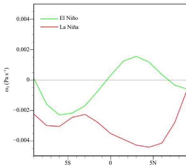
Fig. 14. Meridional distributions of the regressed vertical p -velocity anomaly ( \omega_3 ; \text{Pa s}^{-1} ) at 700 hPa averaged over 130^{\circ} – 150^{\circ}\text{E} for EP El Niño (green) and La Niña (red) winters. The regression was based on the time series of the OLR anomaly at the reference point ( 5^{\circ}\text{S} , 95^{\circ}\text{E} ).
