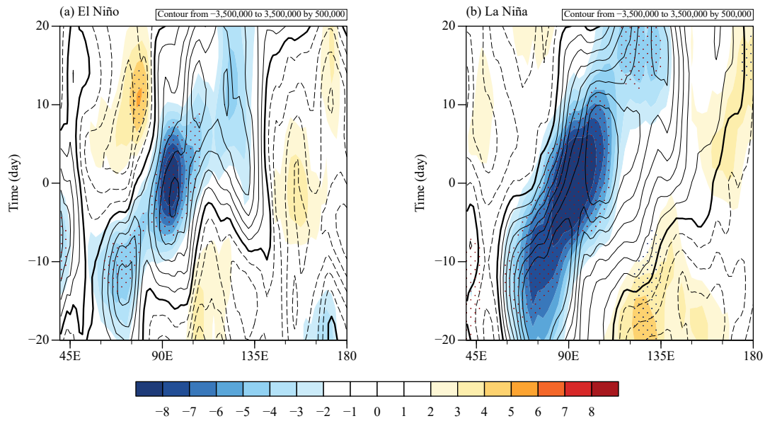
Fig. 3. The Hovmöller diagram of the regressed OLR (shaded; W m^{-2} ) and column-integrated MSE (contour; J m^{-2} ) anomalies averaged over 20^{\circ}S – 20^{\circ}N for (a) EP El Niño and (b) La Niña winters from Days -20 to 20 . The regression was based on the OLR anomaly at 5^{\circ}S , 95^{\circ}E . The OLR anomalies that pass the significant test at 95% confidence level are stippled.
