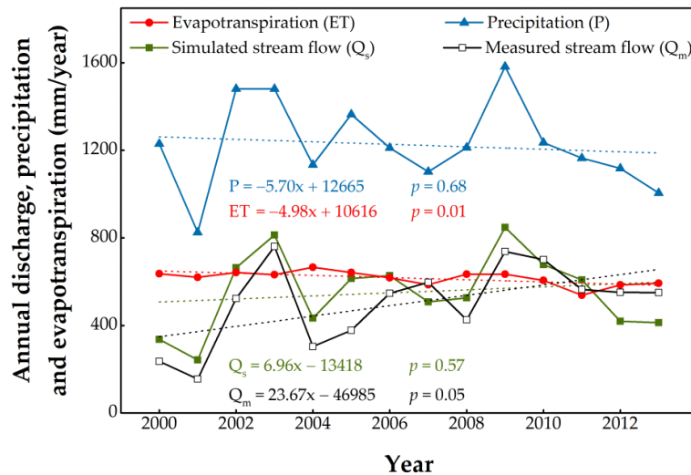
Figure 11. Changes of annual measured stream flow ( Q_m ), simulated stream flow ( Q_s ), evapotranspiration (ET), and precipitation (P) for the Qinhuai River basin from 2000 to 2013.
