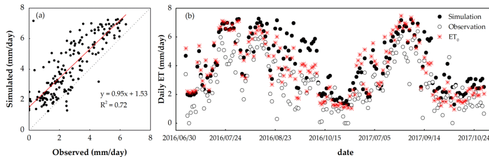
Figure 4. Comparisons between model simulated with observed daily evapotranspiration (ET) in Lishui paddy rice fields during rice growing season (from 30 June 2016 to 2 November 2016 and from 24 June 2017 to 30 October 2017): (a) scatter pot; and (b) time series comparisons of the daily simulated paddy ET derived from the MIKE SHE model, ground observed paddy ET, and average basin reference ET ( ET_0 ).
