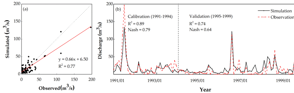
Figure 3. Monthly discharge simulated by the MIKE SHE model versus observed discharge at Wudingmen gauging station: (a) scatter plot for the period from 1991 to 1999; and (b) simulated (continuous line) and observed (dotted line) monthly hydrographs for the calibration (1991–1994) and validation (1995–1999).
